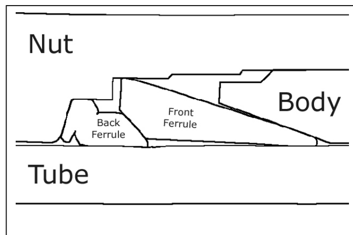
Figure 10: Swagelok SAF 2507 tube fitting after make-up.
