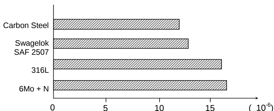
Figure 5: Thermal expansion, per °C (20-100 °C)
