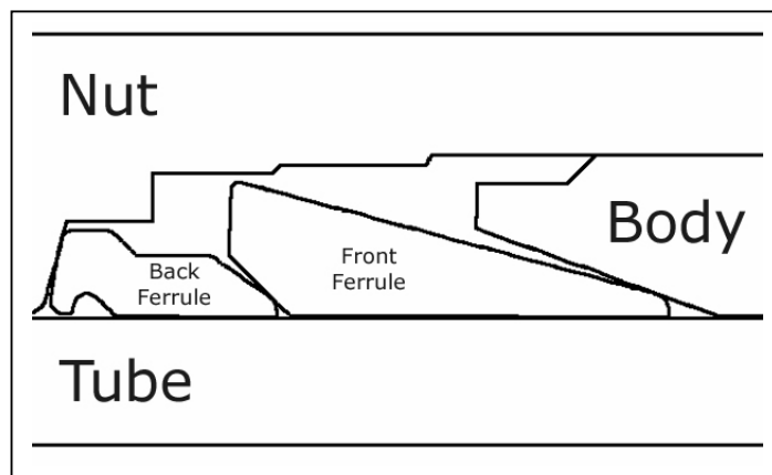
Figure 9: Internals of Swagelok SAF 2507 tube fitting before make-up.
